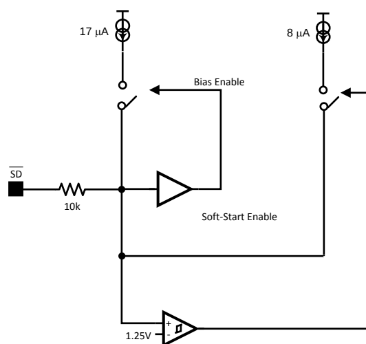
Figure 27. \overline{\text{SD}} Pin Logic
