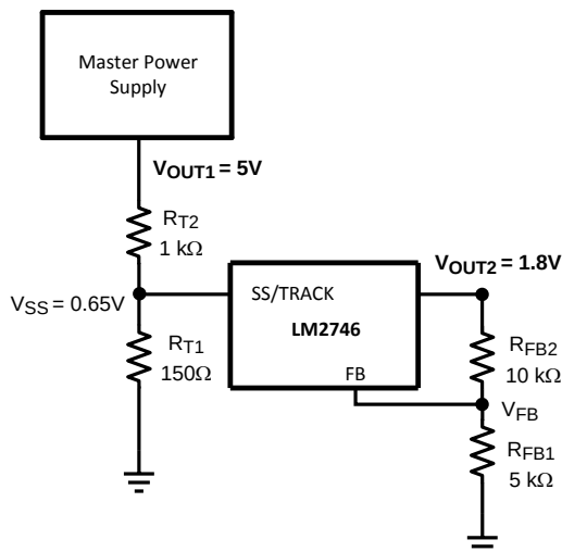
Figure 22. Tracking Circuit
